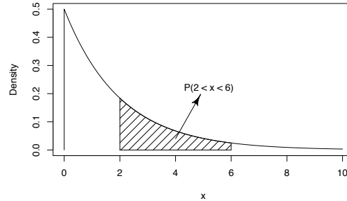
FIGURE 5.6: The Exponential(0.5) Distribution
