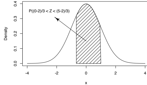
FIGURE 6.3: The Standard Normal Distribution
