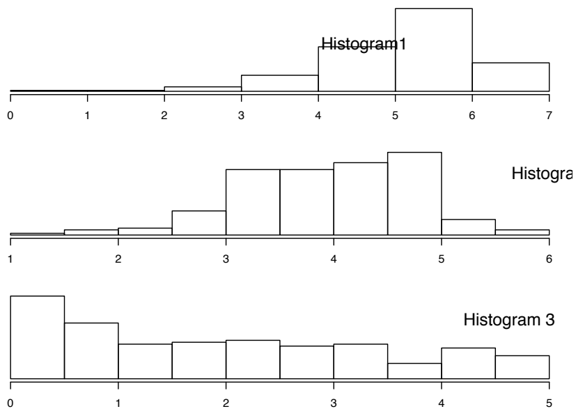
FIGURE 3.3: Three Histograms
