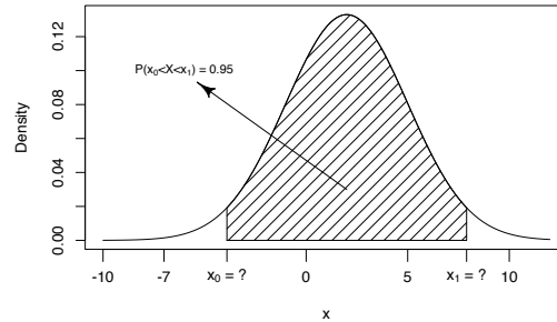
FIGURE 6.5: Central 95% of the Normal(2,9) Distribution
