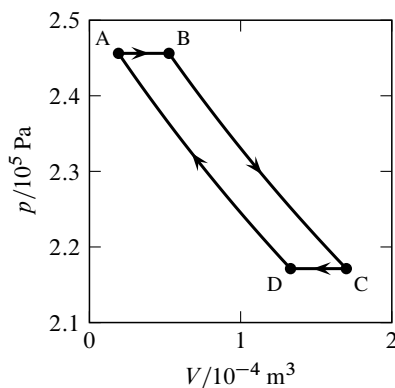
Figure 4.4 Indicator diagram for a Carnot engine using \text{H}_2\text{O} as the working substance. In this example, T_h = 400 \text{ K} , T_c = 396 \text{ K} , \epsilon = 1/100 , w = -1.0 \text{ J} . In state A, the system consists of one mole of \text{H}_2\text{O}(\text{l}) . The processes (all carried out reversibly) are: A \rightarrow B , vaporization of 2.54 \text{ mmol H}_2\text{O} at 400 \text{ K} ; B \rightarrow C , adiabatic expansion, causing vaporization of an additional 7.68 \text{ mmol} ; C \rightarrow D , condensation of 2.50 \text{ mmol} at 396 \text{ K} ; D \rightarrow A , adiabatic compression returning the system to the initial state.
