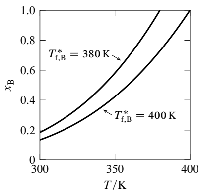
Figure 12.6 Ideal solubility of solid B as a function of T . The curves are calculated for two solids having the same molar enthalpy of fusion ( \Delta_{\text{fus},B}H = 20 \text{ kJ mol}^{-1} ) and the values of T_{f,B}^* indicated.
