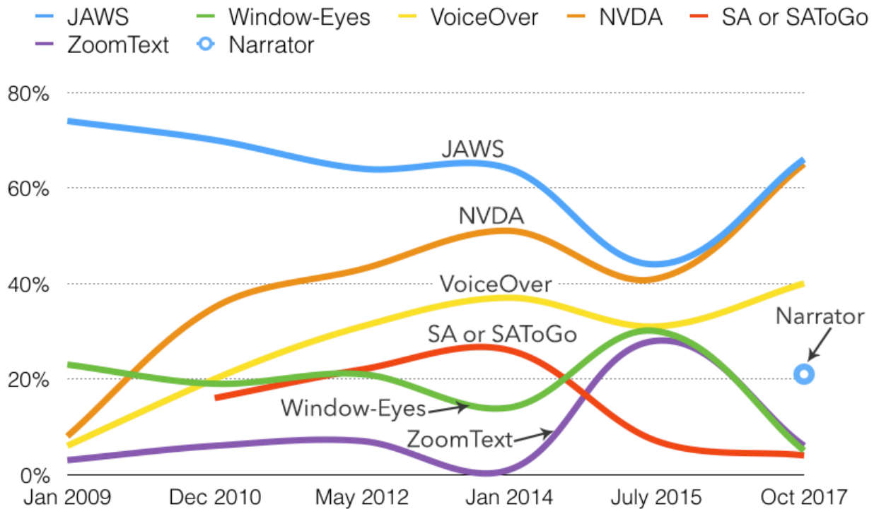
Figure: Screen readers commonly used, usage patterns
